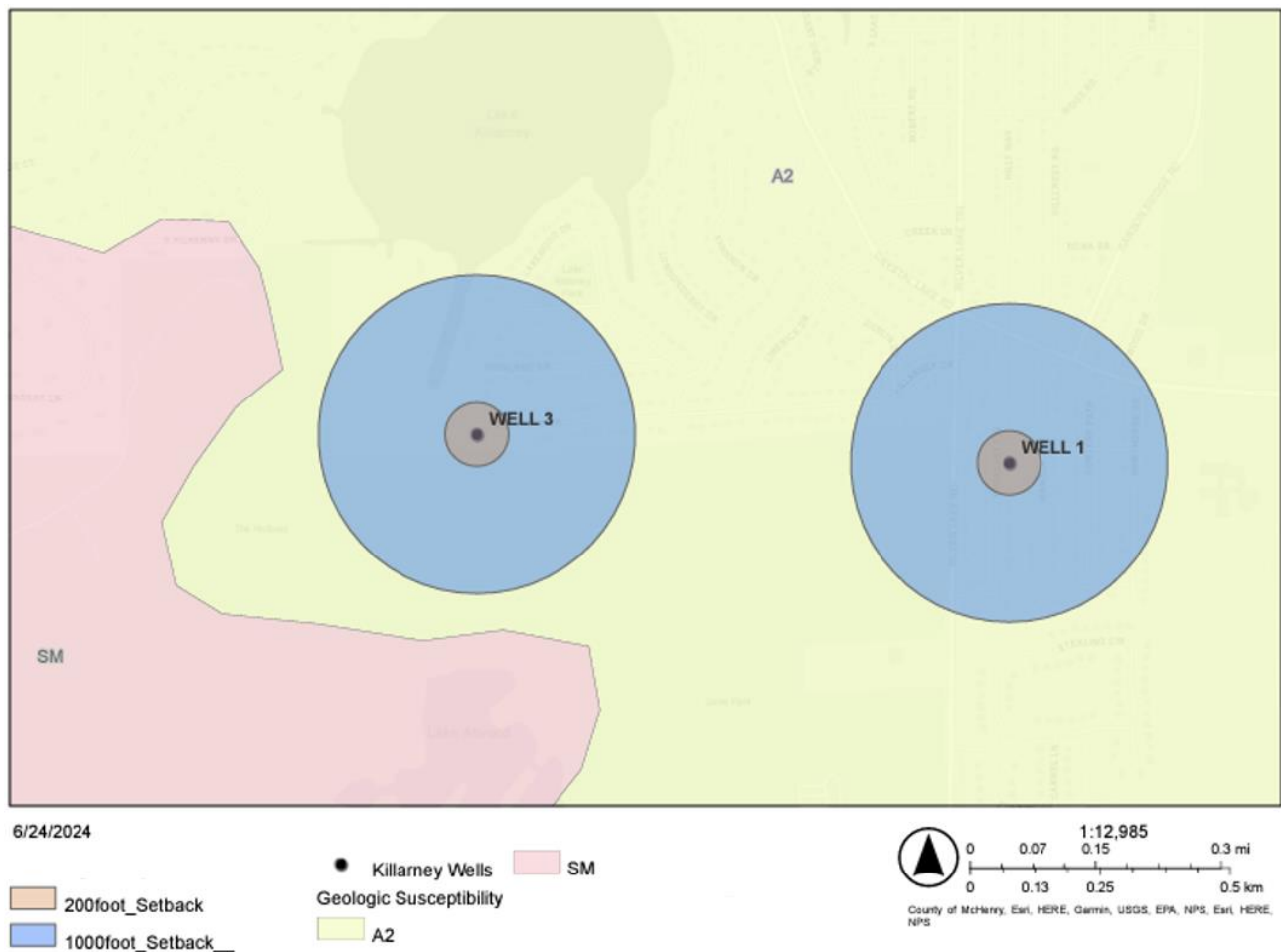
Exhibit 3-4: Groundwater Susceptibility
