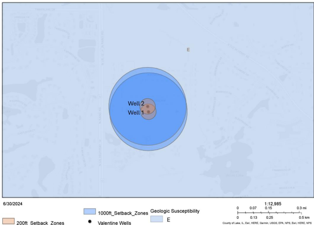
Exhibit 3-4: Groundwater Susceptibility
