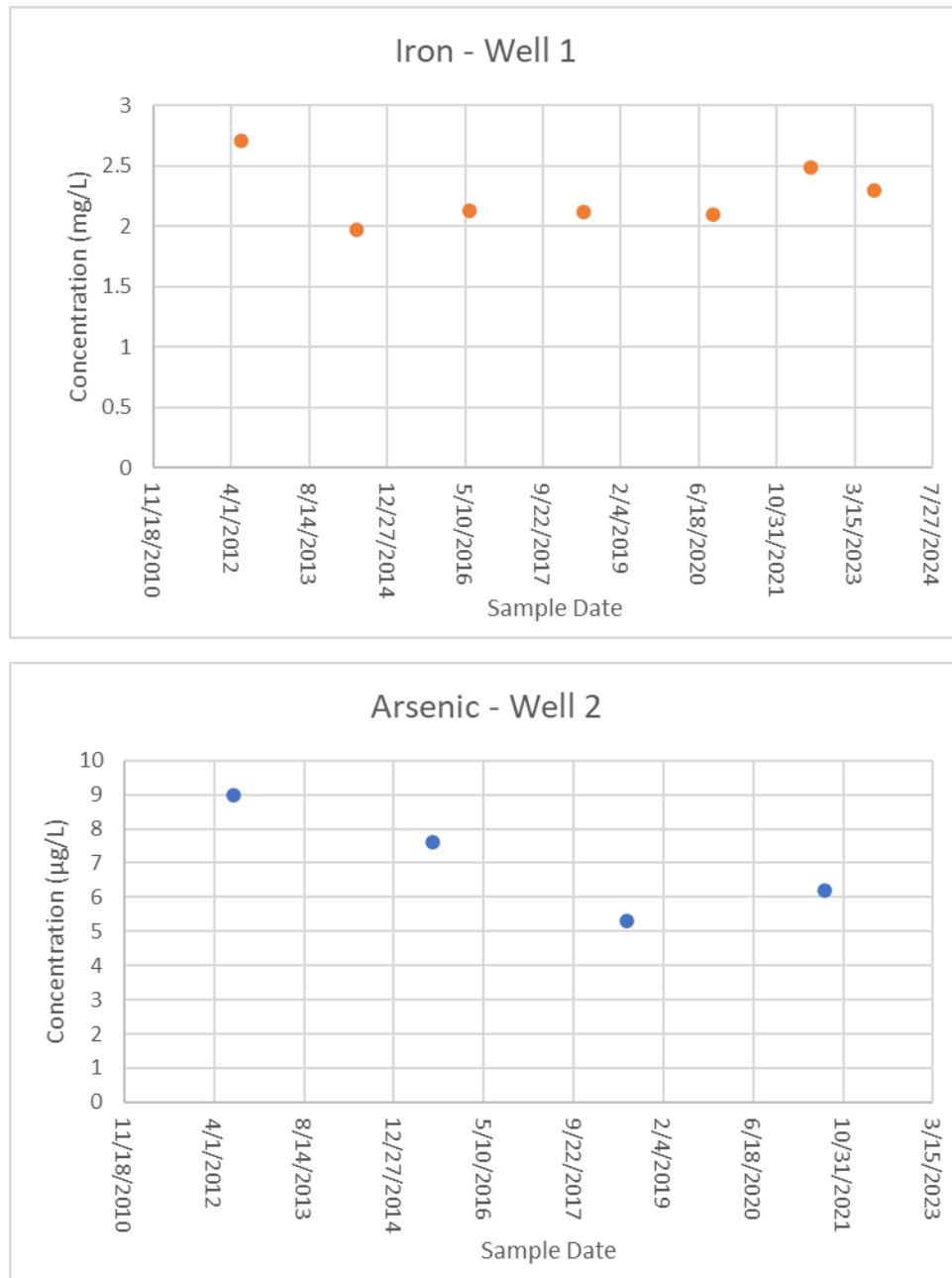
Exhibit 3-2: Iron and Arsenic Concentration Trend
